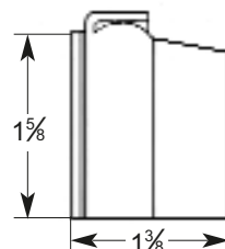
No. 52 Welded For Inside Angle Iron
